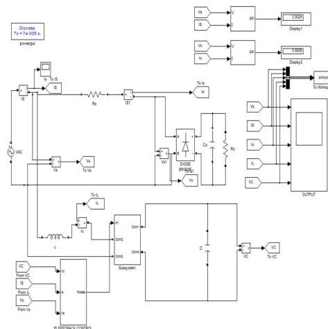
Figure.9. SAPF with PI controllers
