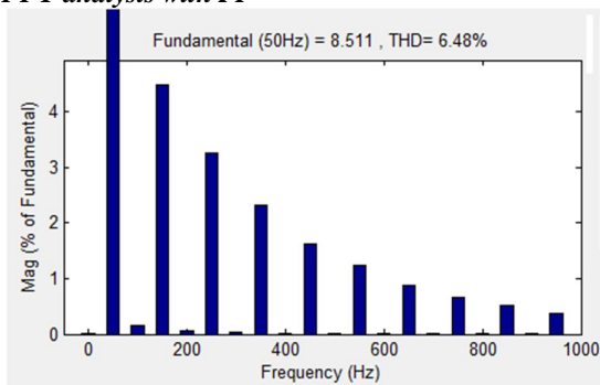
Figure 11. FFT analysis of source current with PI controller
