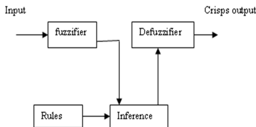
Figure.7. Fuzzy controller block diagram
