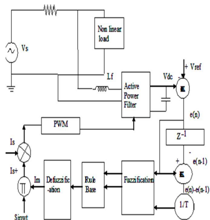
Figure.8. Structure of the fuzzy for APF controller
