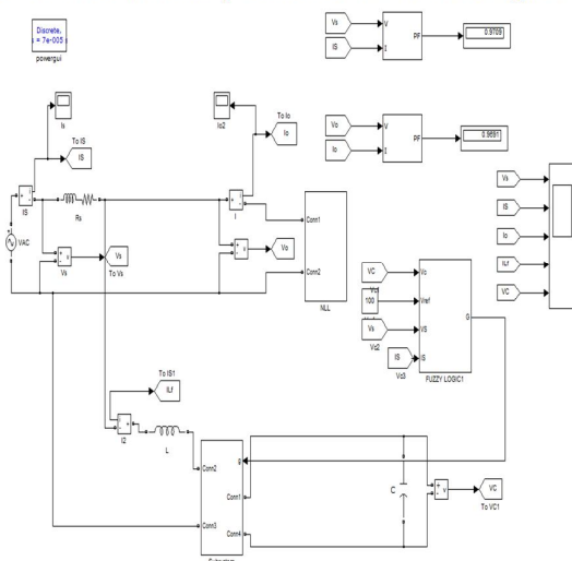
Figure 12. SAPF with fuzzy logic controller
