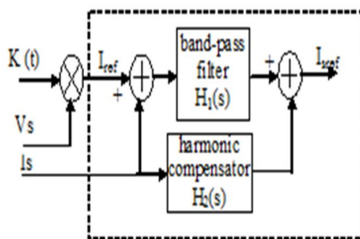
Figure.5. Reference Generator
