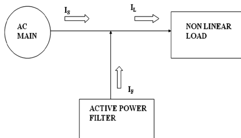
Figure.1. Basic concept shunt active filter
