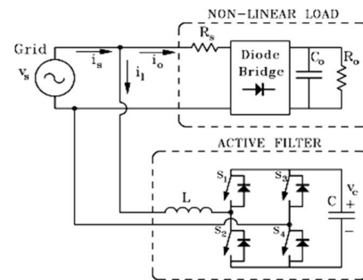
Figure 2. Shunt APF with non-linear load and the full-bridge converter
