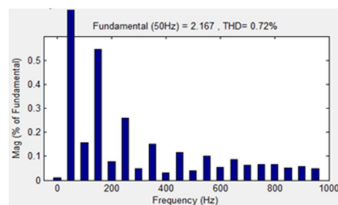
Figure 14. FFT analysis of source current with FLC
